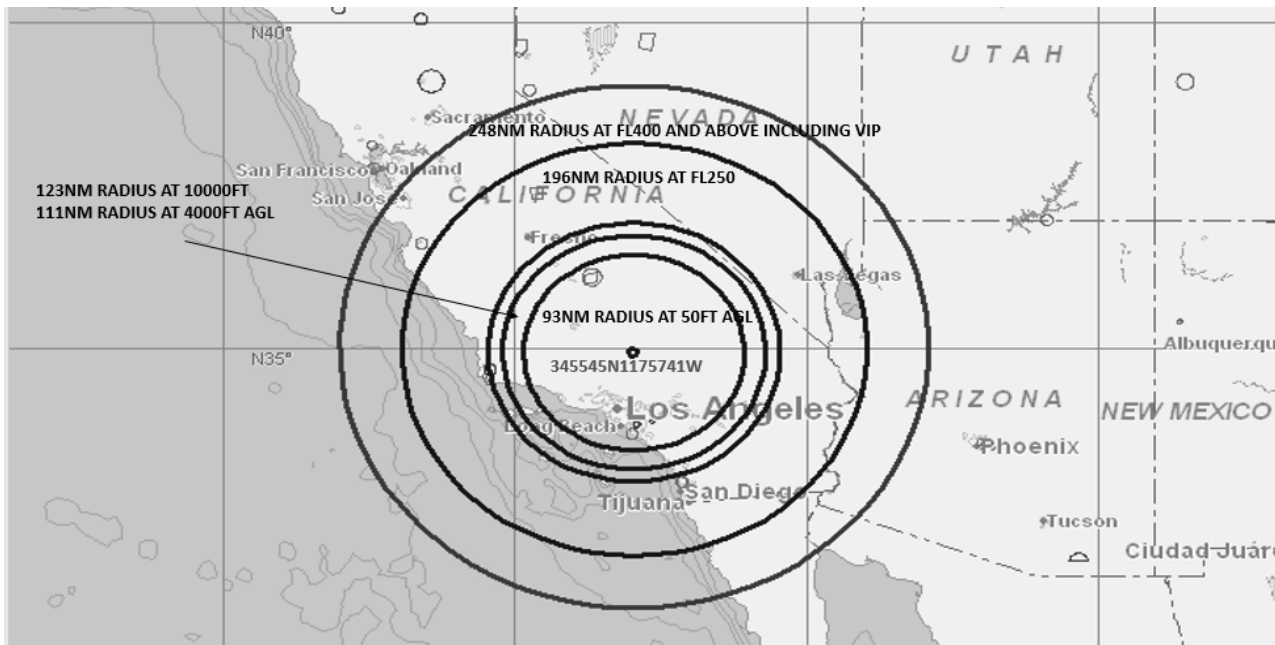
EDW 18-04 GPS INTERFERENCE TESTING
